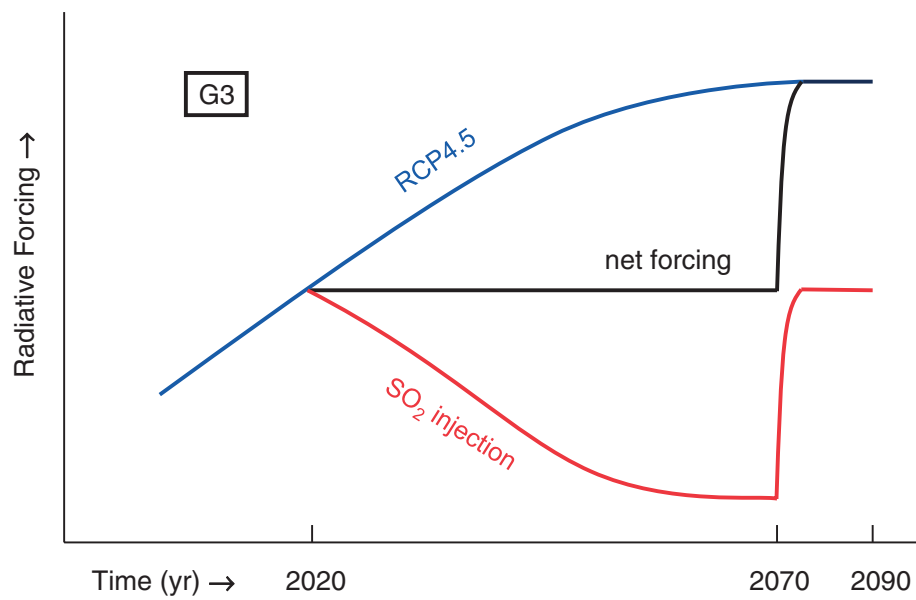
Figure 1: Time evolution of radiative forcing under RCP4.5 and under the G3 geoengineering scenario
