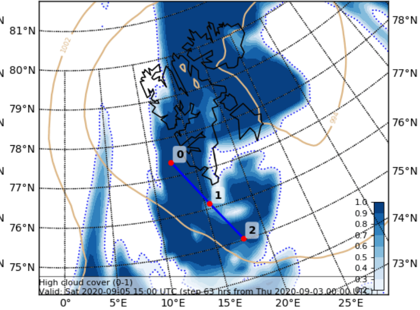
Cloud Cover (0-1) (High Cloud Cover) Valid: Sat 2020-09-05 15:00 UTC (step 63 hrs from Thu 2020-09-03 00:00 UTC)
