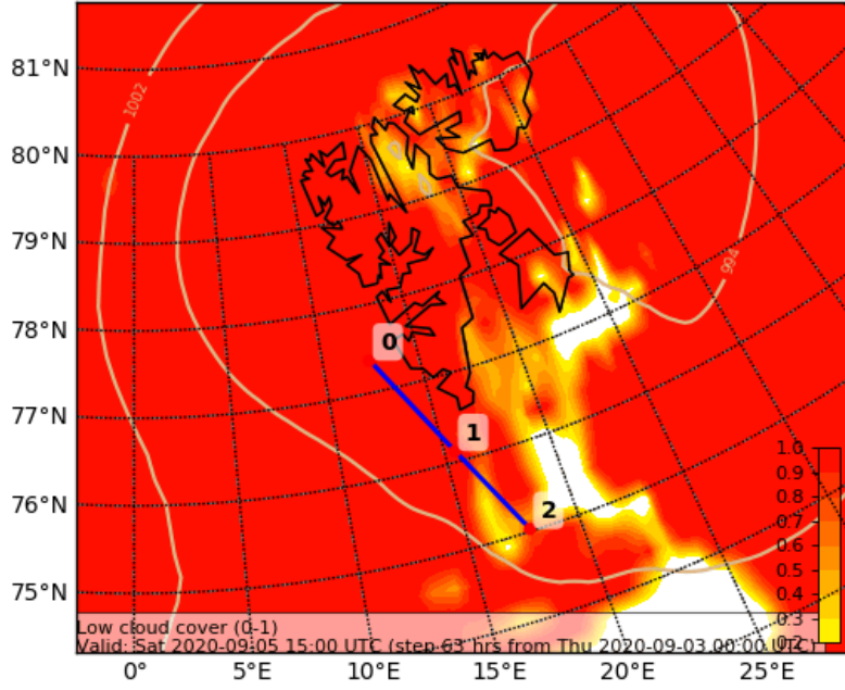
Cloud Cover (0-1) (Low Cloud Cover) Valid: Sat 2020-09-05 15:00 UTC (step 63 hrs from Thu 2020-09-03 00:00 UTC)
