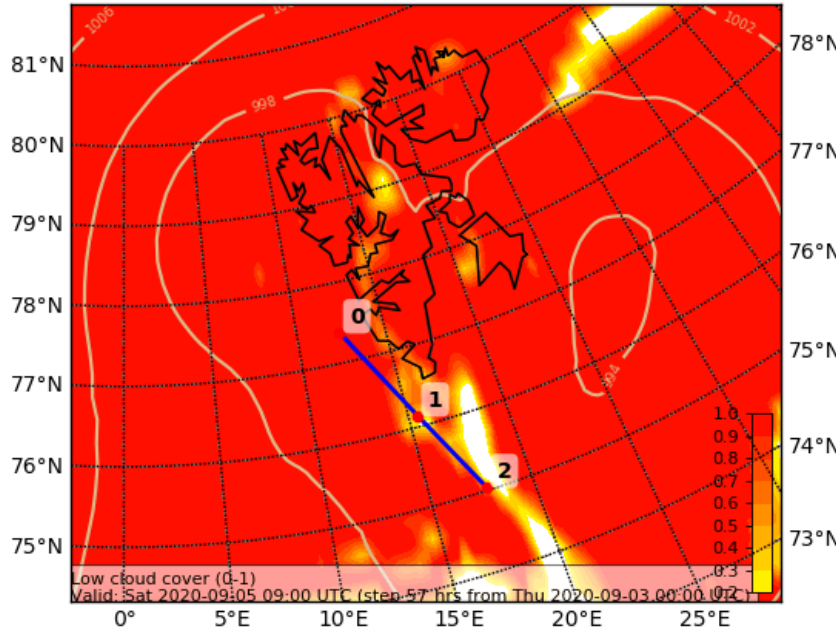
Cloud Cover (0-1) (Low Cloud Cover)
