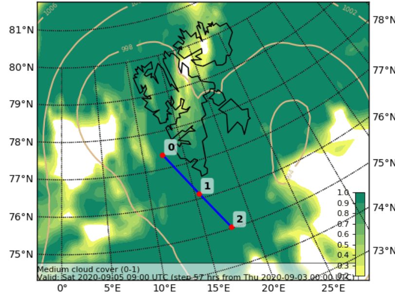
Cloud Cover (0-1) (Medium Cloud Cover)
