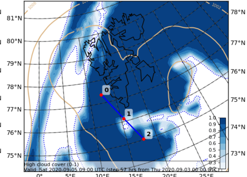
Cloud Cover (0-1) (High Cloud Cover)
