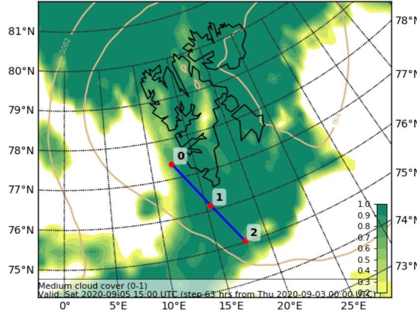
Cloud Cover (0-1) (Medium Cloud Cover) Valid: Sat 2020-09-05 15:00 UTC (step 63 hrs from Thu 2020-09-03 00:00 UTC)
