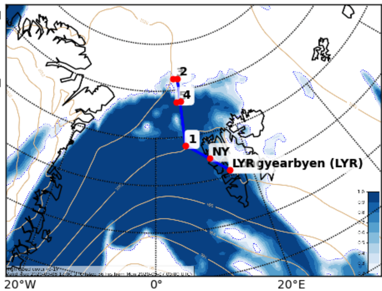
Cloud Cover (0-1) (High Cloud Cover) Valid: Di 2020-09-08 12:00 UTC (step 36 hrs from Mo 2020-09-07 00:00 UTC)
