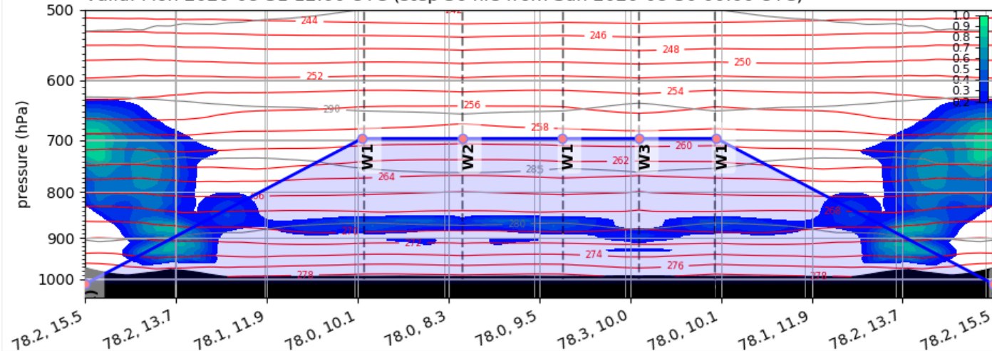
Cloud Cover (0-1) Vertical Section Valid: Mon 2020-08-31 12:00 UTC (step 36 hrs from Sun 2020-08-30 00:00 UTC)
