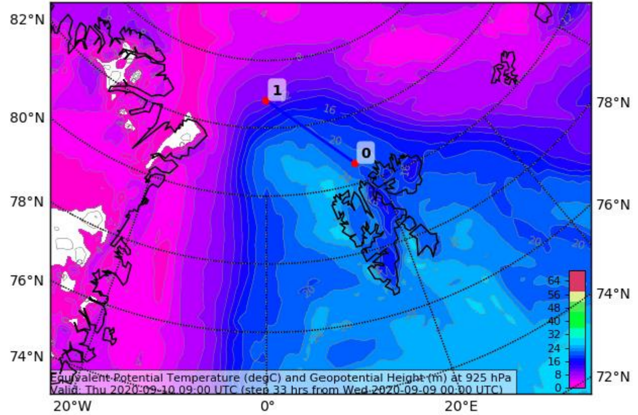
Equivalent Potential Temperature (degC) and Geopotential Height (m) at 925 hPa Valid: Thu 2020-09-10 09:00 UTC (step 33 hrs from Wed 2020-09-09 00:00 UTC)
