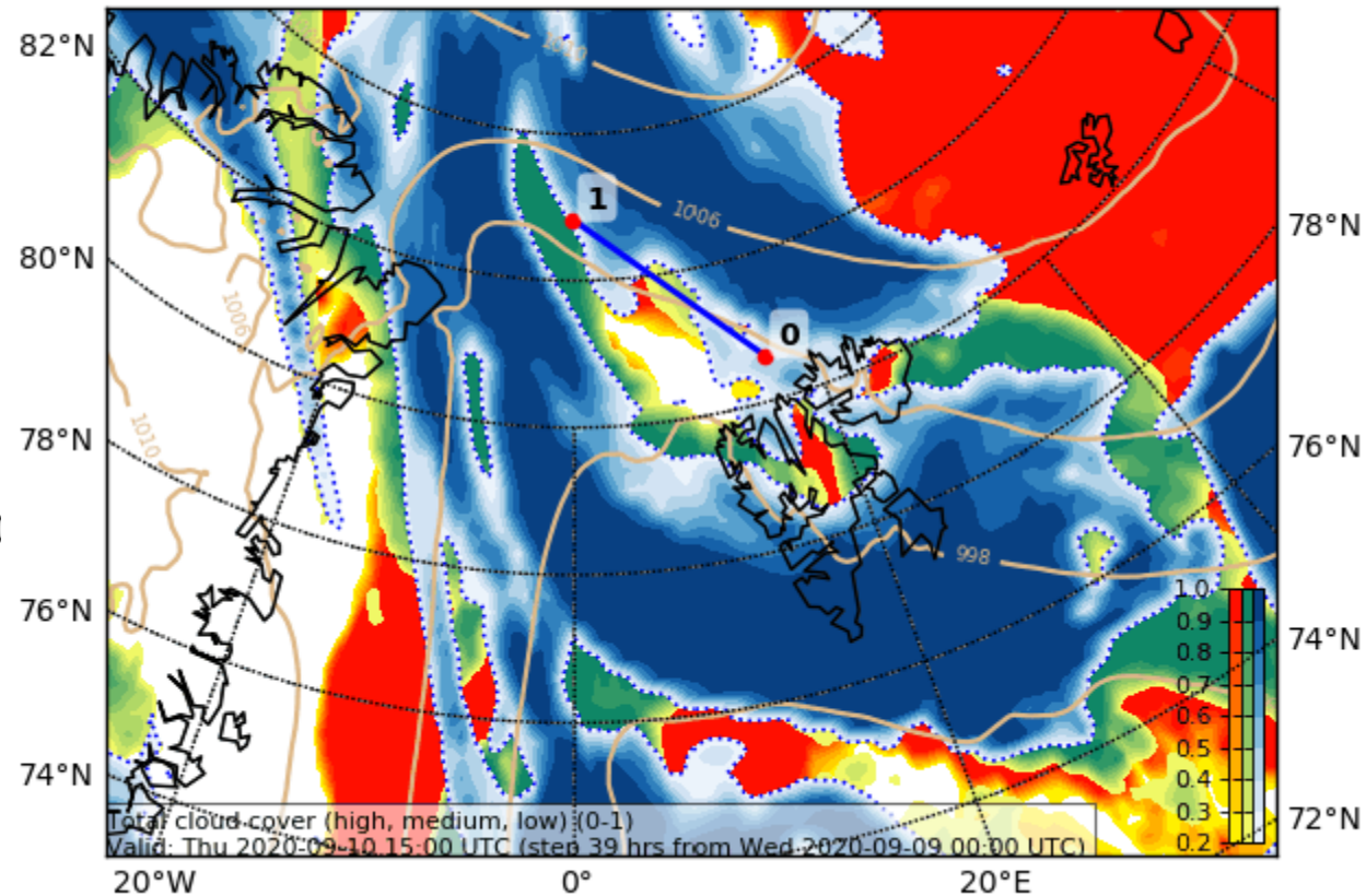
Cloud Cover (0-1) (Total Cloud Cover) Valid: Thu 2020-09-10 15:00 UTC (step 39 hrs from Wed 2020-09-09 00:00 UTC)
