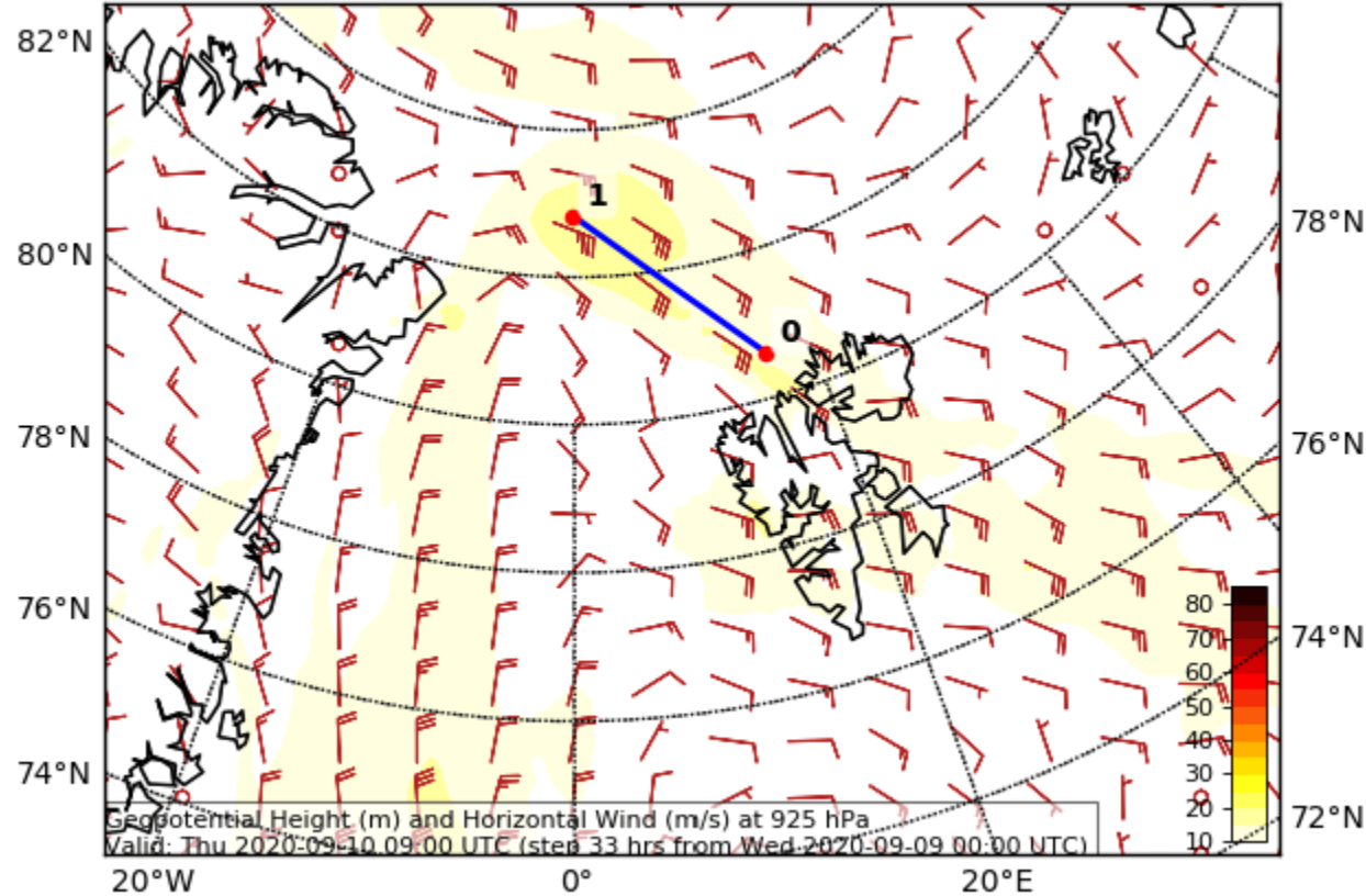
Geopotential Height (m) and Horizontal Wind (m/s) (Wind Speed 10-16 m/s) Valid: Thu 2020-09-10 09:00 UTC (step 33 hrs from Wed 2020-09-09 00:00 UTC)
