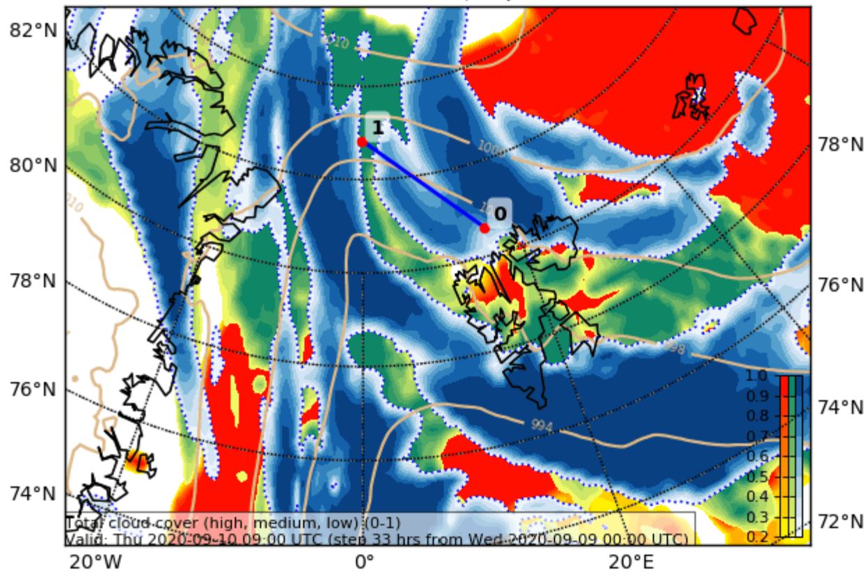
Cloud Cover (0-1) (Total Cloud Cover) Valid: Thu 2020-09-10 09:00 UTC (step 33 hrs from Wed 2020-09-09 00:00 UTC)
