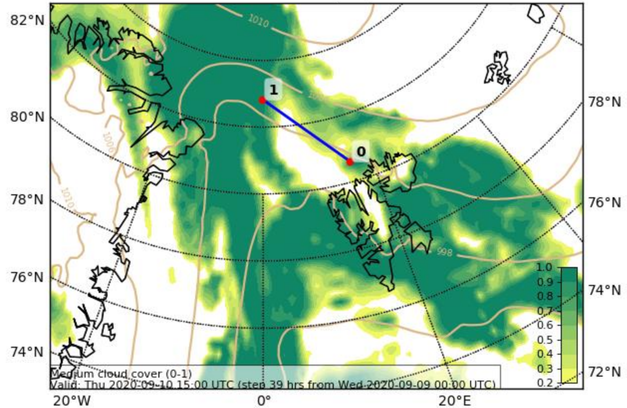
Cloud Cover (0-1) (Medium Cloud Cover) Valid: Thu 2020-09-10 15:00 UTC (step 39 hrs from Wed 2020-09-09 00:00 UTC)
