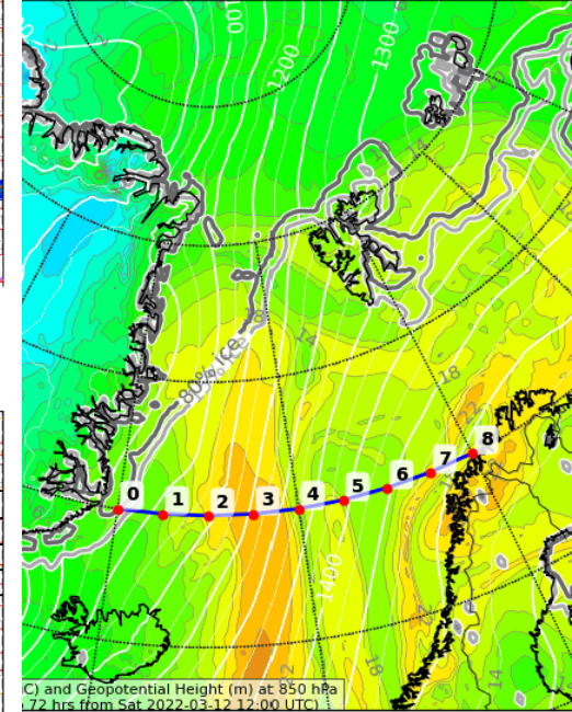
Potential (degC) and Geopotential Height (m) at 850 hPa Valid: 2022-03-15T12:00:00Z (initialisation: 2022-03-12T12:00:00Z)
