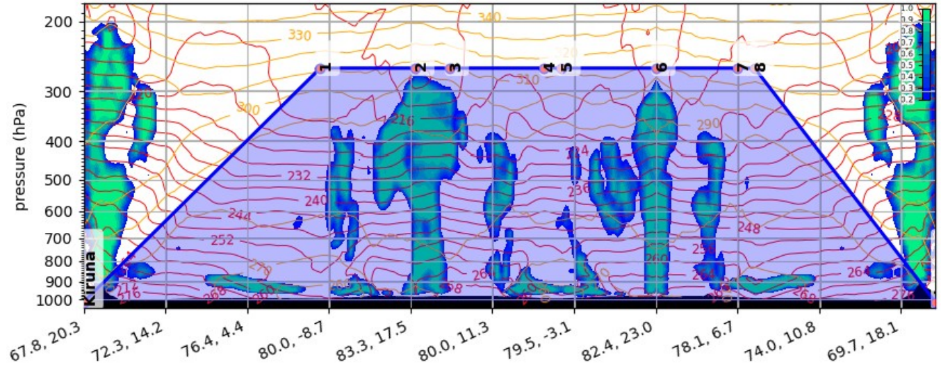
Cloud Cover (0-1) Vertical Section Valid: 2022-03-19T12:00:00Z (initialisation: 2022-03-16T12:00:00Z)
