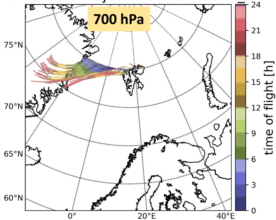
24h forward trajectories 20210326 12
