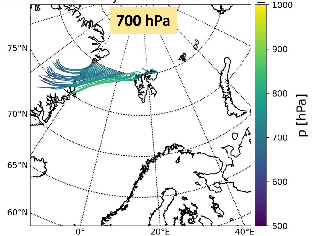
24h forward trajectories 20210326 12
