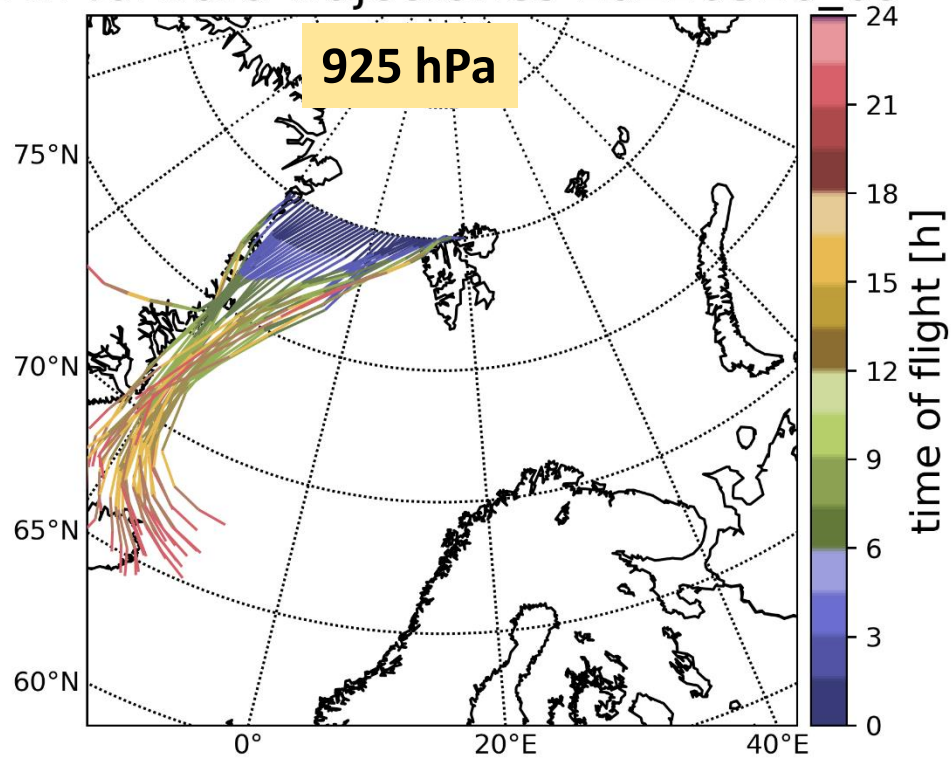
24h forward trajectories 20210326 09
