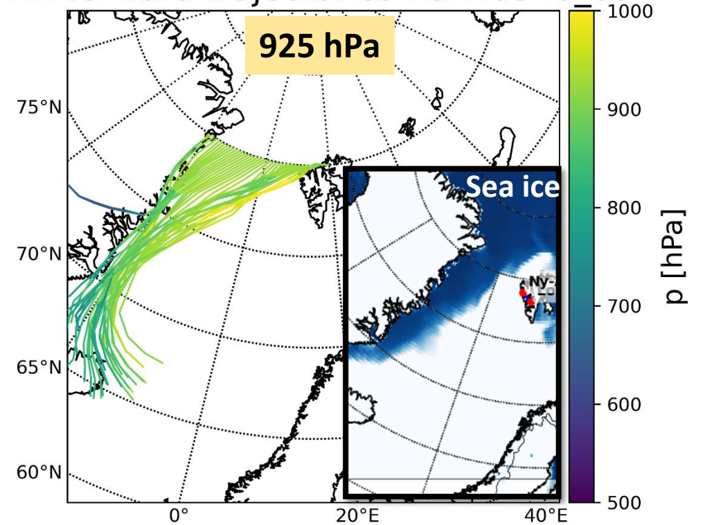
24h forward trajectories 20210326 09
