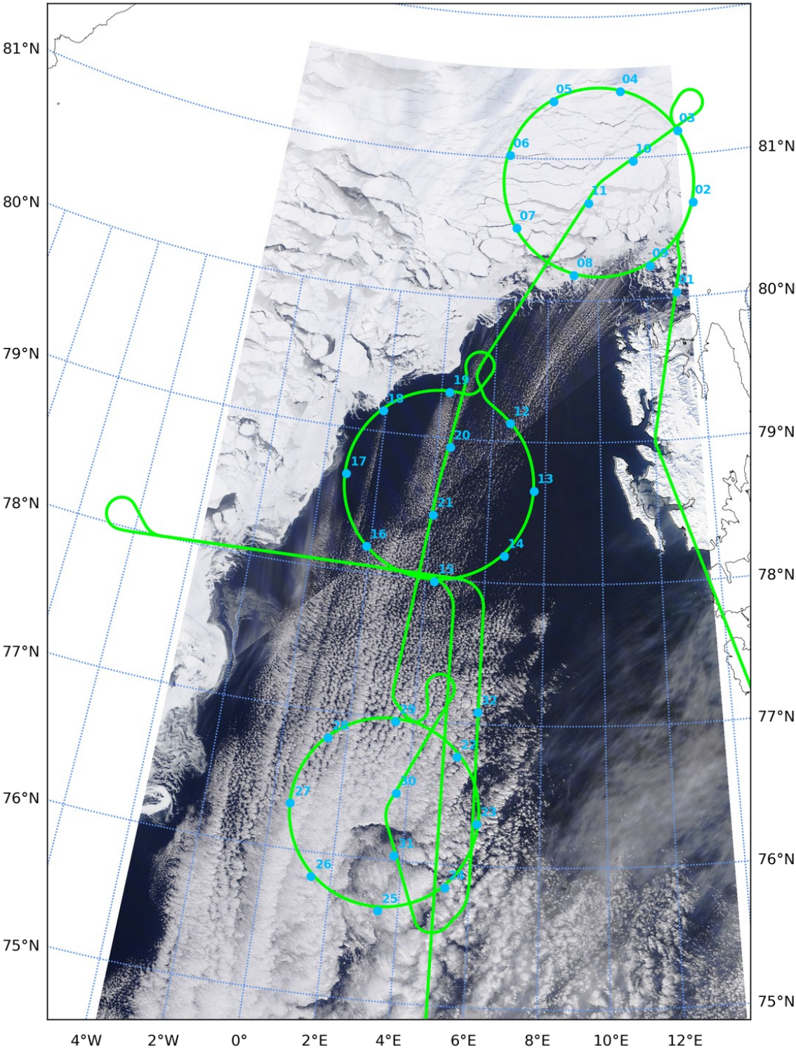
Fig. 2: MODIS Terra true color satellite image of clouds and sea ice in the Fram Strait on 30 March 2022. The HALO flight path is show in green. Dropsonde launch locations are indicated in blue. The low level air mass transitioned from stable over the sea ice via shallow well-mixed at cloud onset to stratocumulus topped mixed layers in the south.
