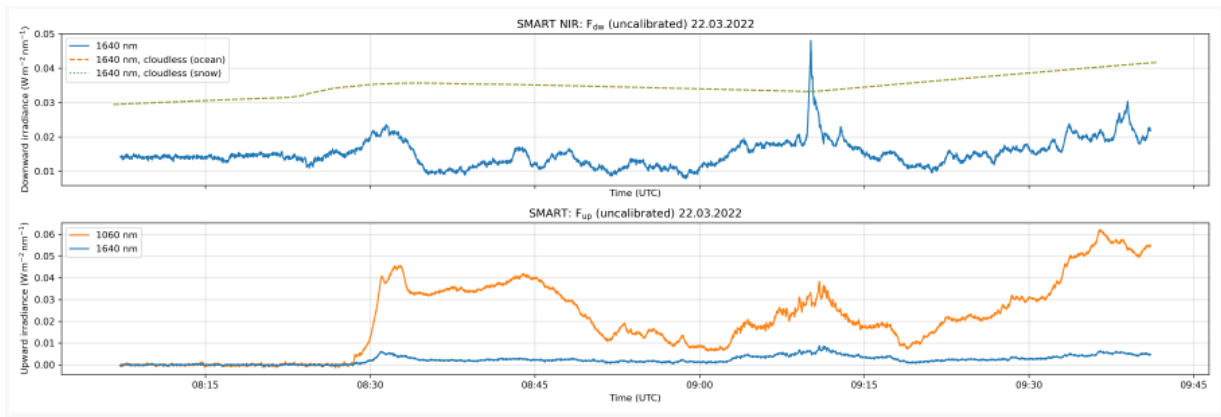
SMART spectral radiances.
